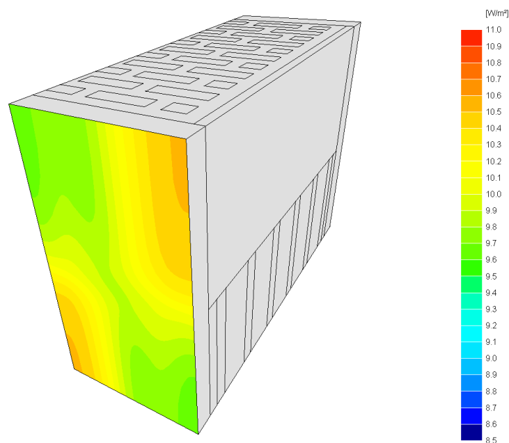
Figure 5. Heat flow density at the internal surface.
